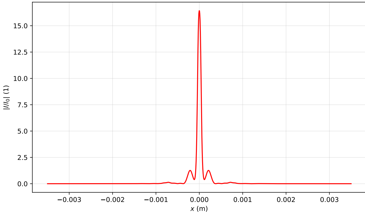
Intensity profile I(x, y = 0, z = 0.955)/I_0 , P_{in}=6.5P_{cr} , artificial time
